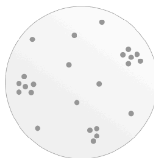
But our results suggest that many features form "lumps" — a kind of anisotropic superposition .
